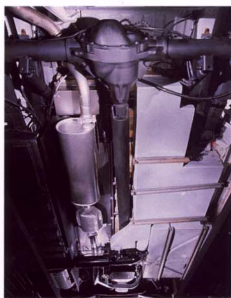
Water tanks fit below the floor which maximizes interior storage space. Locating them between the axles improves weight distribution for better handling.
