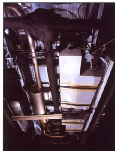
Water tanks are custom made to fit below the floor, which maximizes interior storage space. Locating them between the axles improves weight distribution for better handling.
